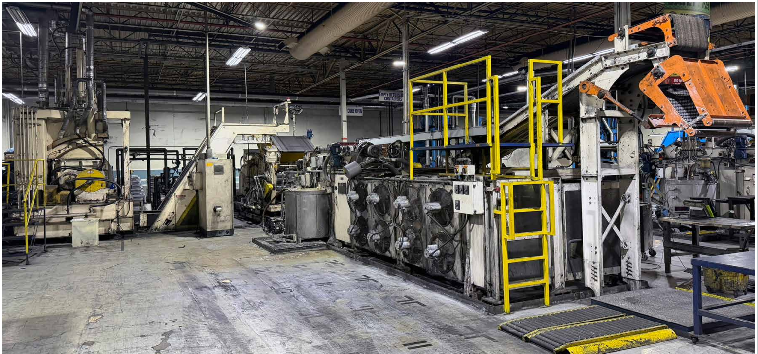
KNEADER Mixing Line
