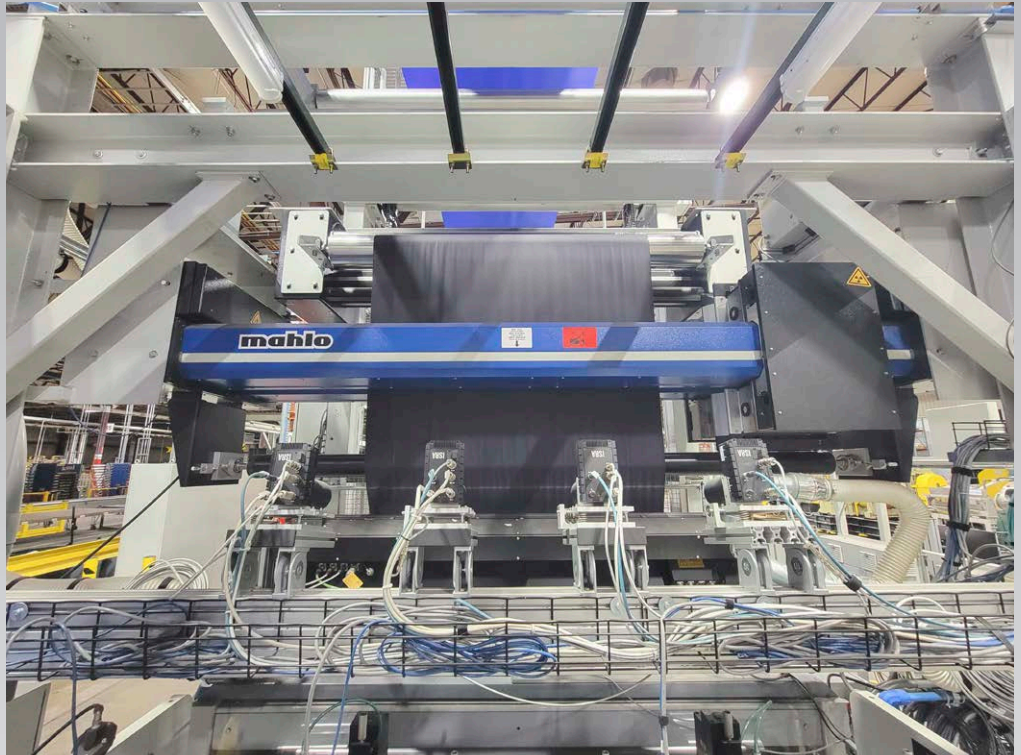
ISRA Surface Vision SMASH Advanced Inspection System
