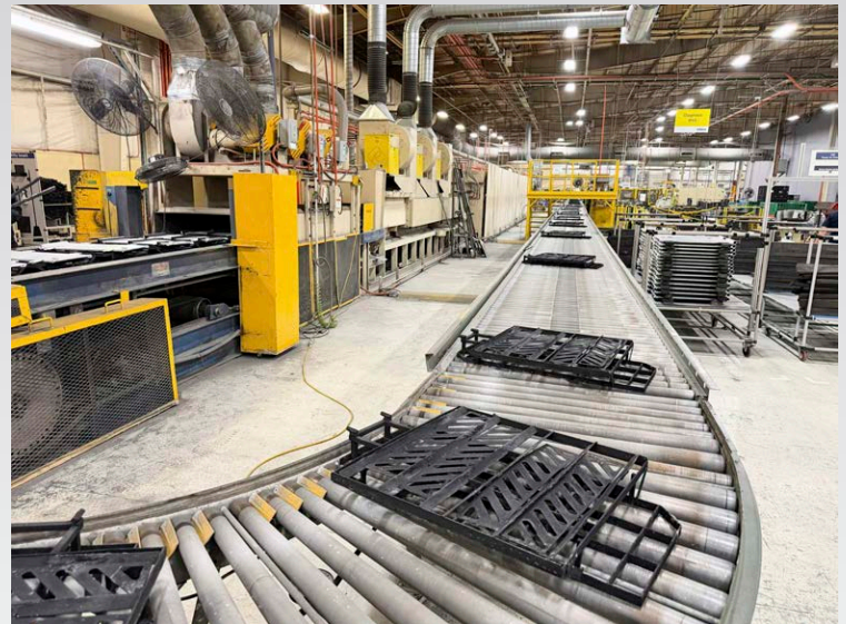
Rogers Model OMB Cab Brazing System (2 of 2)
